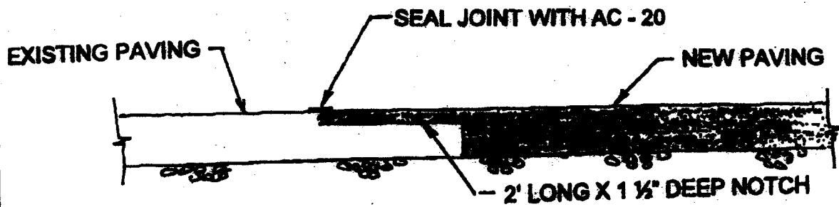
NEW PAVING NOTCH DETAIL SCALE: NONE
