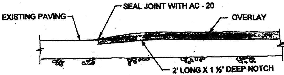
OVERLAY NOTCH DETAIL SCALE: NONE
